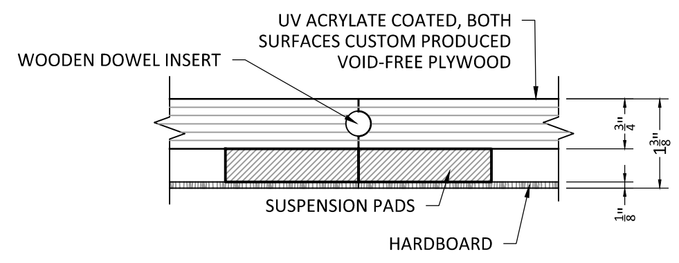
① JOINT DETAIL SCALE: NTS
