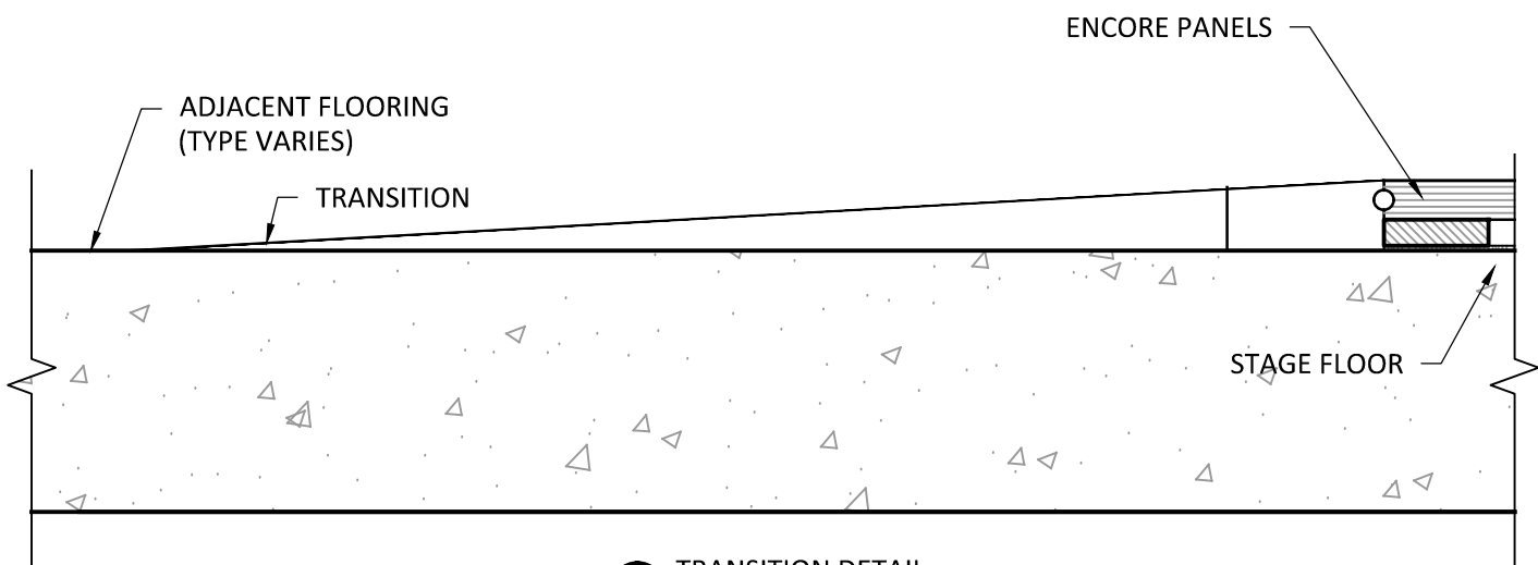
③ TRANSITION DETAIL SCALE: NTS
