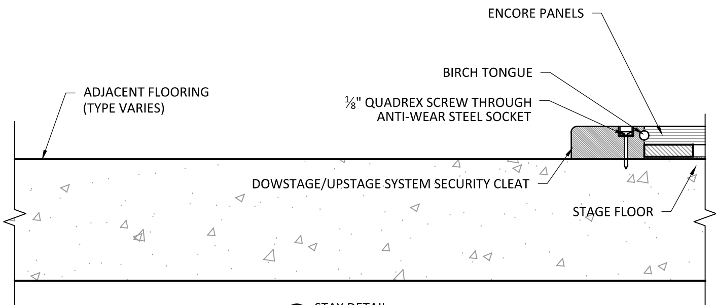
② STAY DETAIL SCALE: NTS
