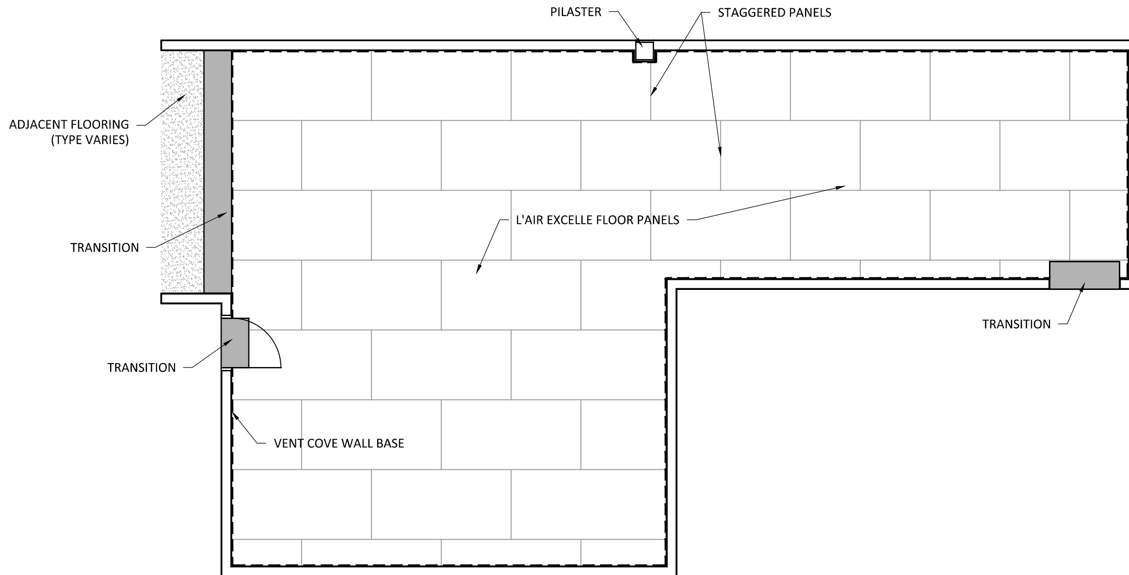
① EXCELLE SUSPENDED FLOORING PANELS SAMPLE PLAN SCALE: 3/16"=1'-0"
