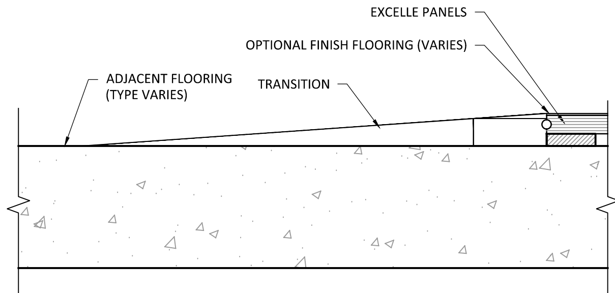
③ TRANSITION DETAIL SCALE: NTS
