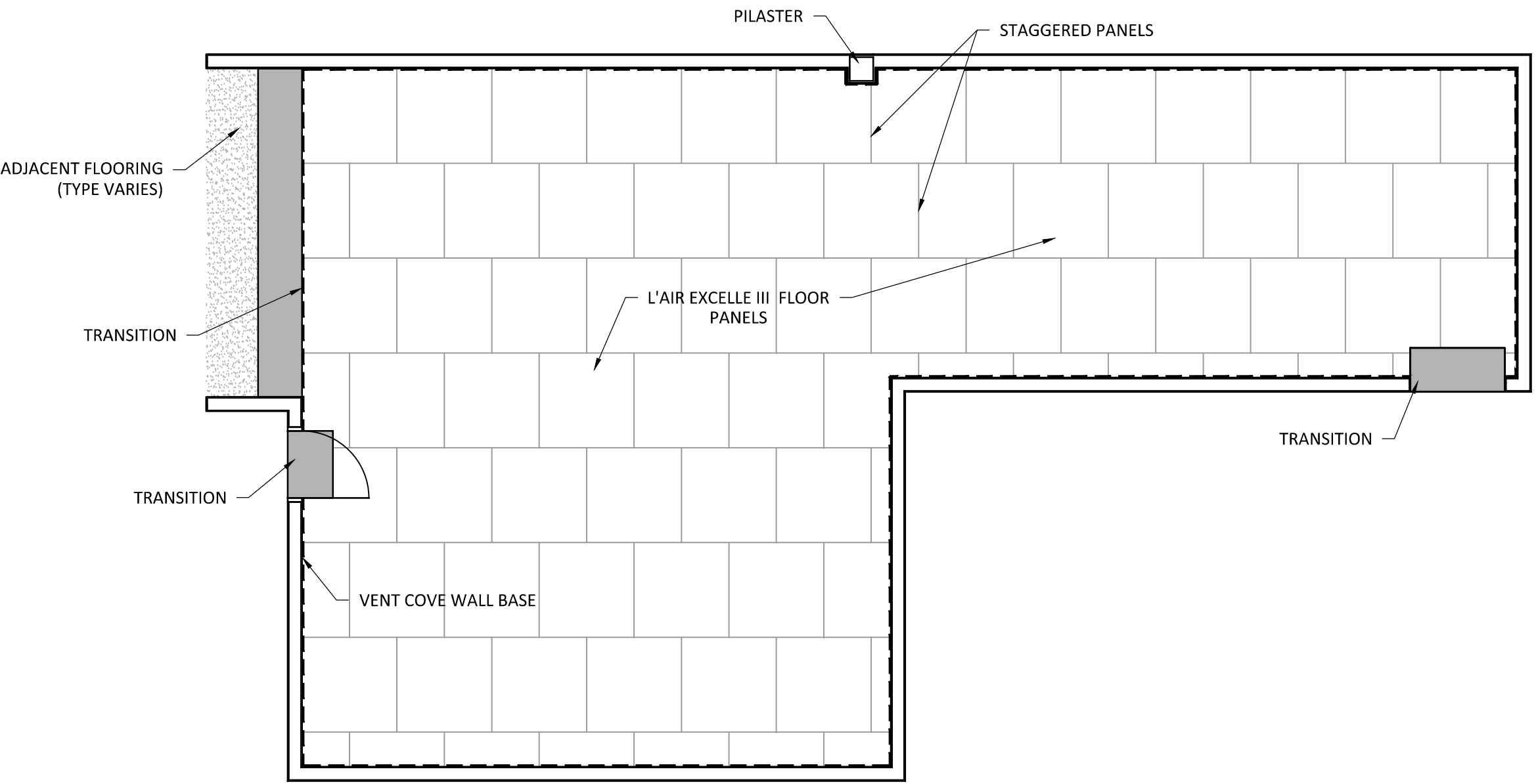
① EXCELLE III SUSPENDED FLOORING PANELS SAMPLE PLAN SCALE: 3/16"=1'-0"
