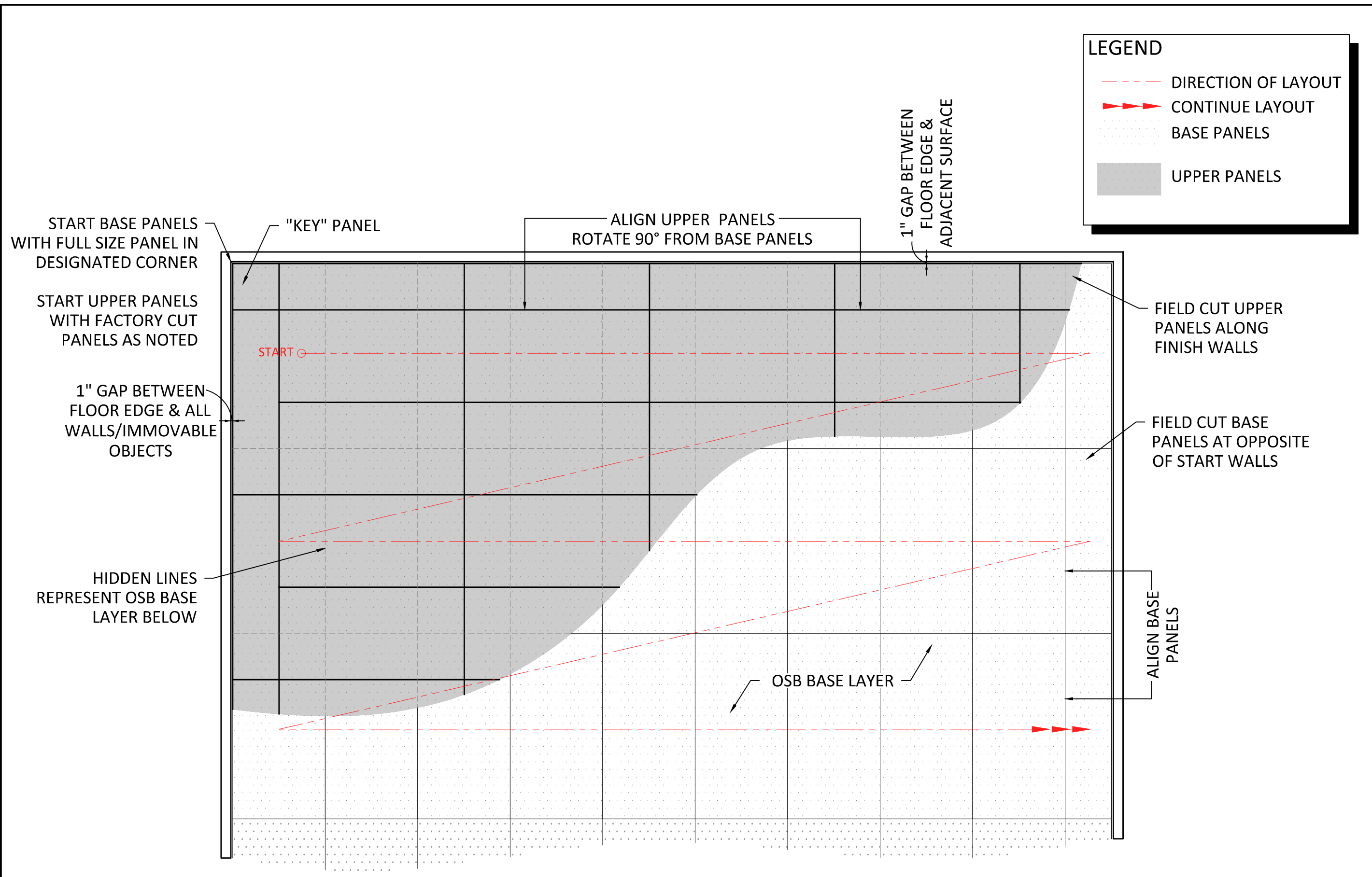
1 EXCELLE IV & VI SPRUNG FLOORING PANEL INSTALLATION SAMPLE PLAN SCALE: 1/4"=1'-0"
