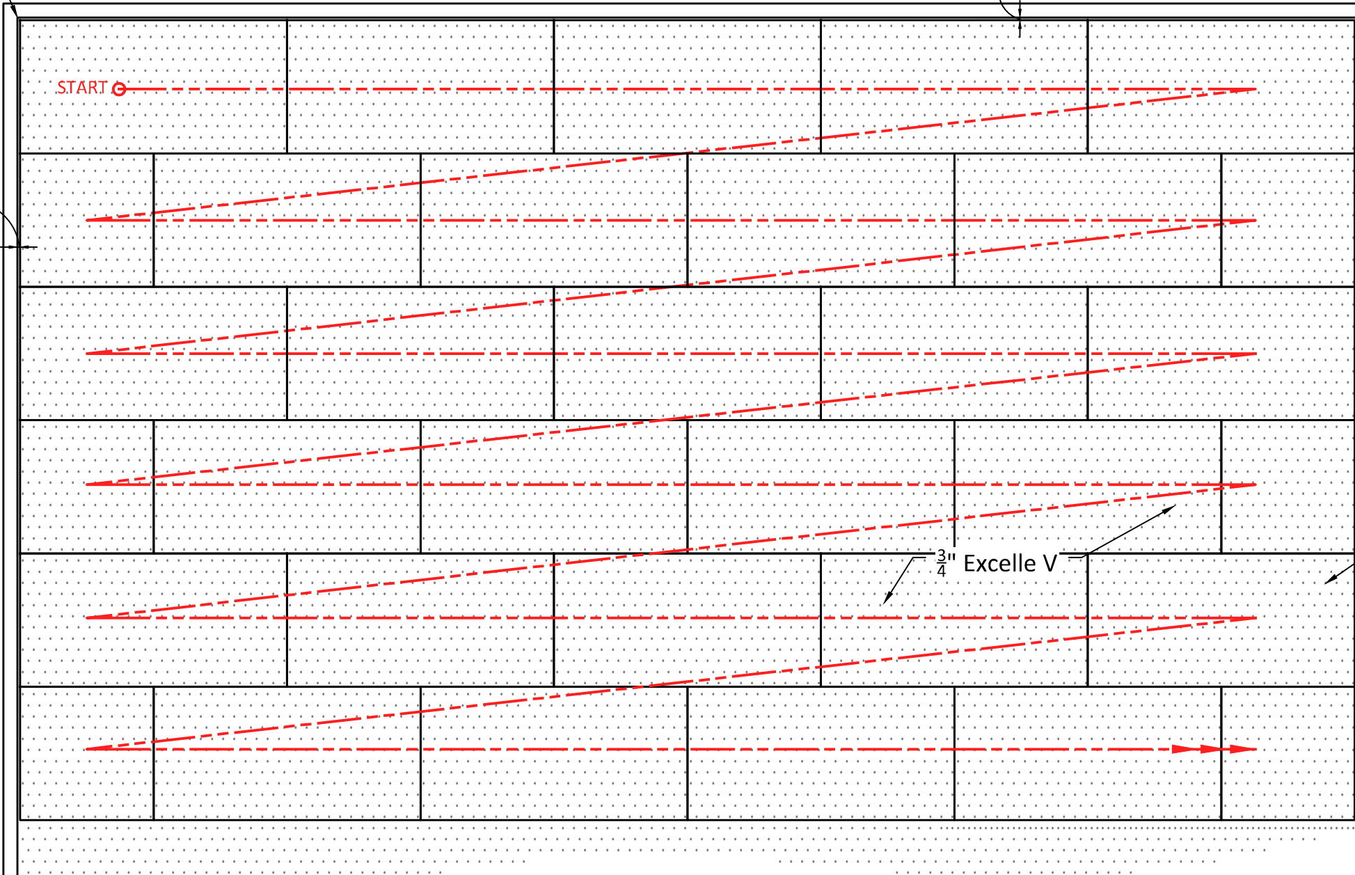
1 EXCELLE V SPRUNG FLOORING PANEL INSTALLATION SAMPLE PLAN SCALE: 1/4"=1'-0"
