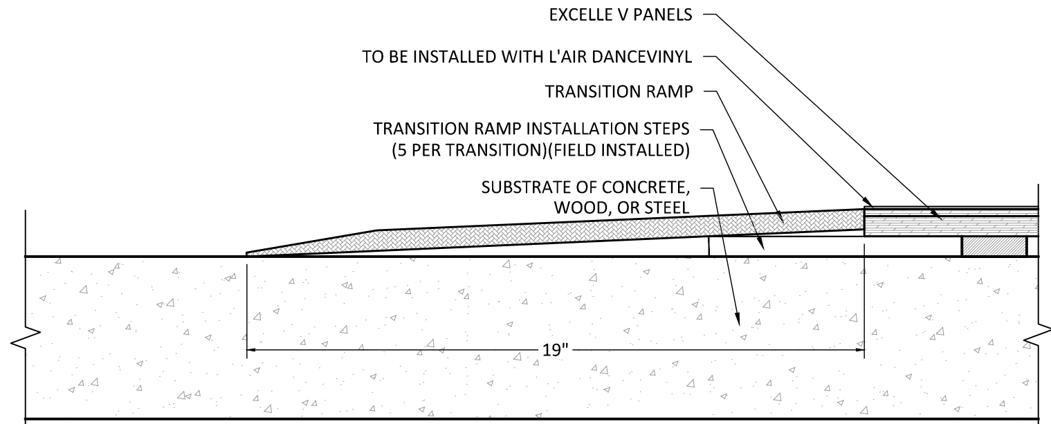
③ TRANSITION DETAIL SCALE: NTS
